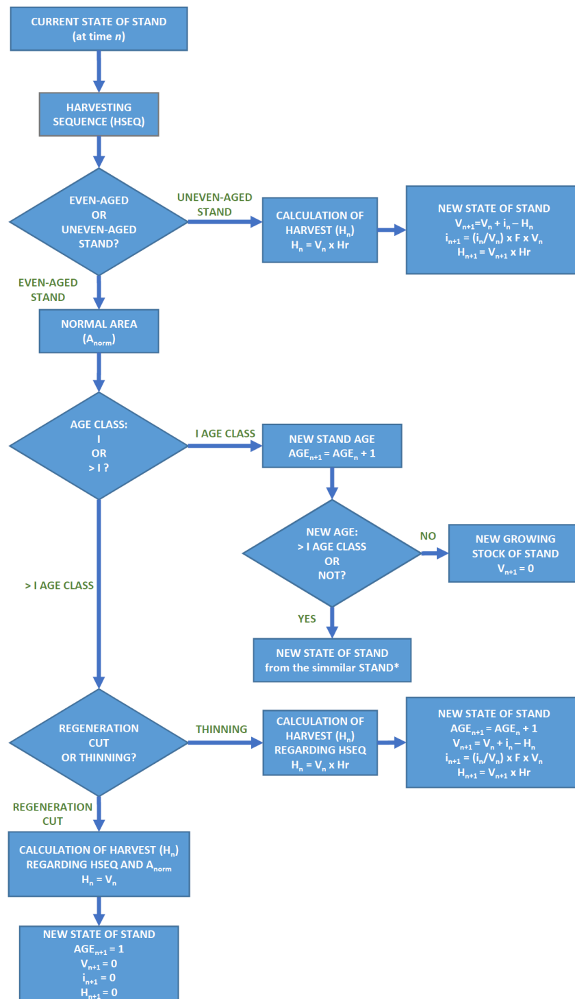
Figure 4.3-5 Flowchart of the model run. H_n – harvest in the year n ( m^3 ), V_n – growing stock in the year n ( m^3 ), H_r – harvesting rates (%), i_n – increment in the year n ( m^3 ), F – factor of age-dependant decrease of increment rate, AGE_n – age of a modelling unit at a year n (years)
