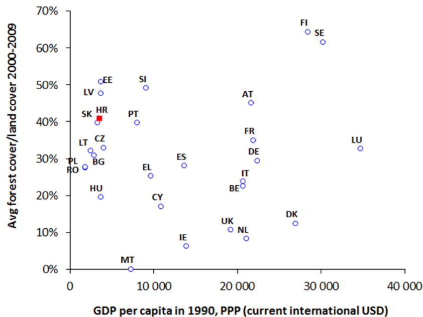
Figure 2.3-2 Average forest cover/land cover 2000-2009 (Source: Materials provided during Regulation negotiations) versus Per capita GDP (Source: UNdata 2018) for the EU countries.
